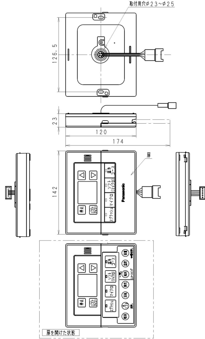
浴室リモコン外形図 ABD-4121ACSKJ3M ABD-4121ACSKJ2M ABD-4121ACSK-JM ABD-4121ACSK-M
