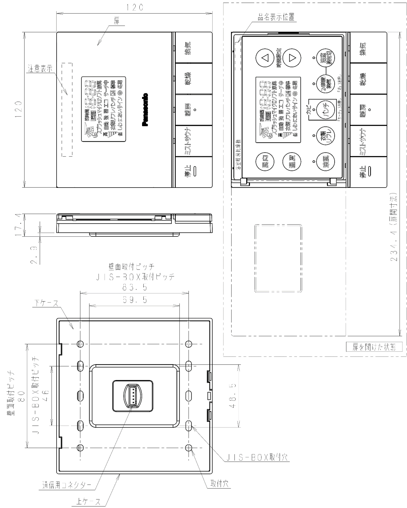
脱衣室リモコン外形図 ABD-4121ACSKJ3M ABD-4121ACSKJ2M ABD-4121ACSK-JM
